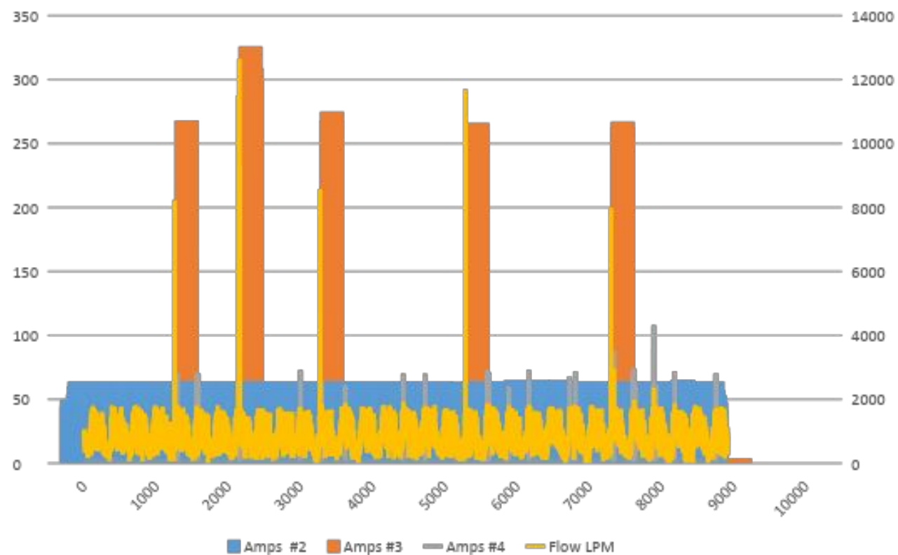
Dec 2020 Flow LPM x 10 & Amps x10
