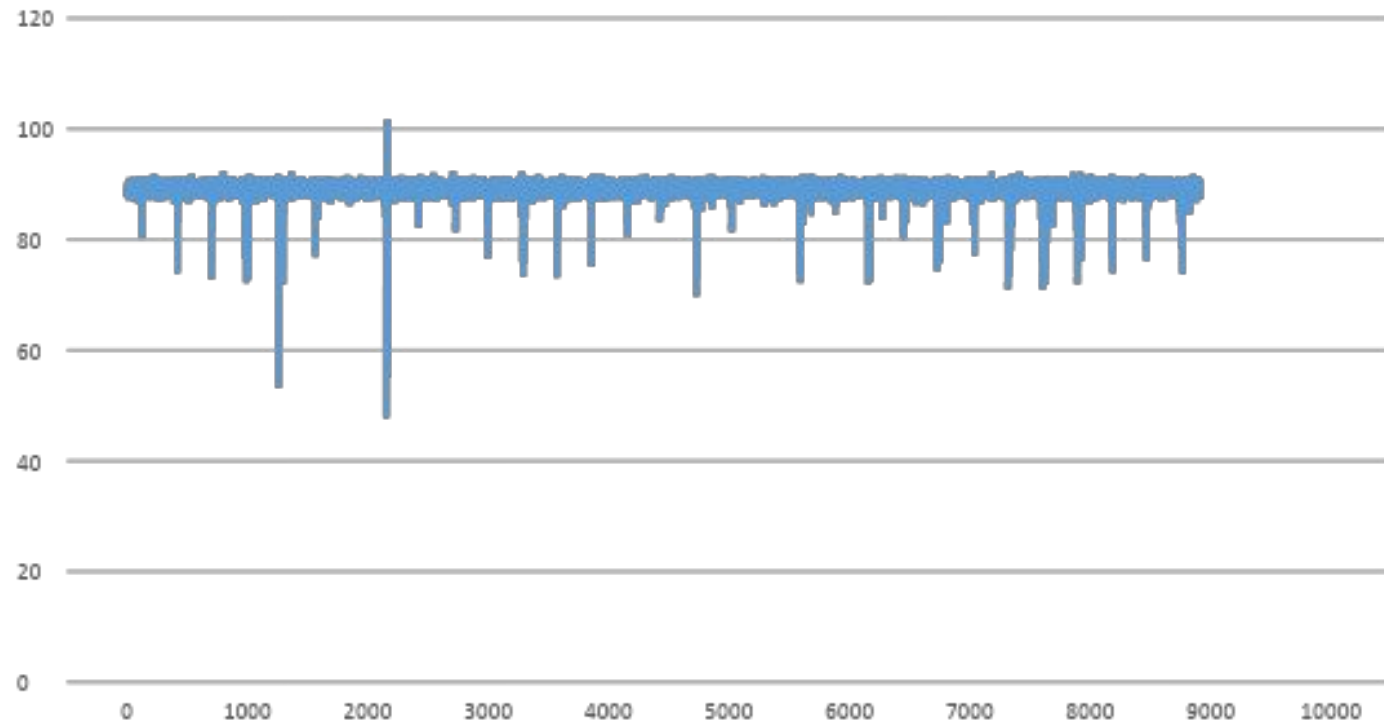
Dec 2020 Discharge pressure PSI
