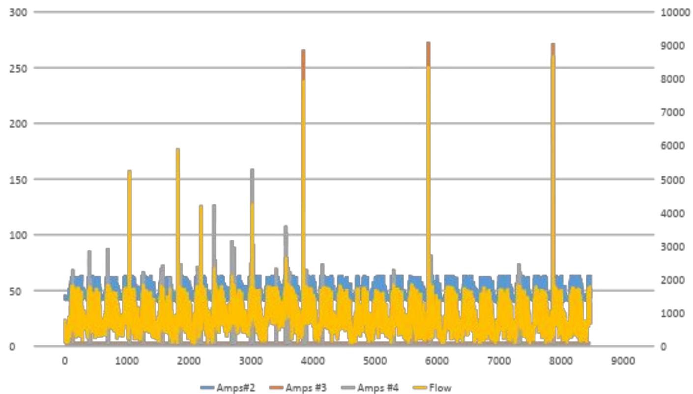
Nov 2020 Flow LPM x 10 & Amps x10
